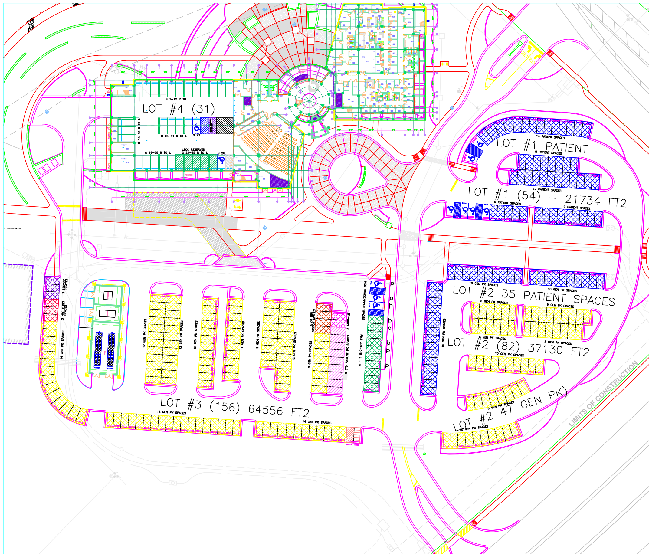
1 ROUND ROCK PARKING PLAN SCALE: 1" = 70'
